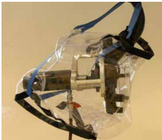
Example of the hydraulic tool applied with guard and catch strap
